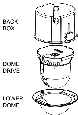
Figure 1. System Components (In-Ceiling Model Shown)
